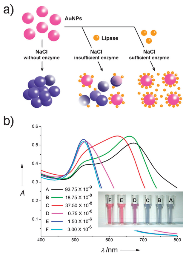
Fig. 1 (a) The diagram of determining the optimal immobilization of lipase-functionalized on gold nanoparticles; (b) variation in UV-Vis absorbance spectra of the AuNPs (2.2 nM) at different concentrations of enzyme after adding salt solution (0.1 mL 10% NaCl solution).
